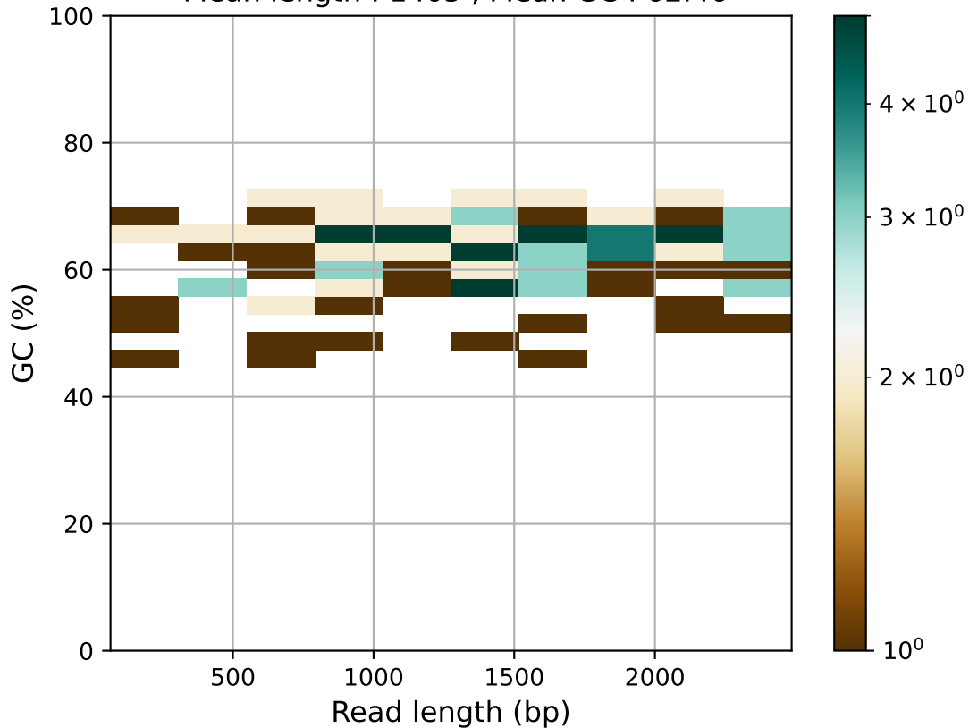
GC % vs length Mean length : 1405 , Mean GC : 62.46
